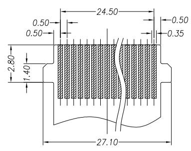
APPLICABLE FPC DIMENSION (THICKNESS: 0.3±0.05)
